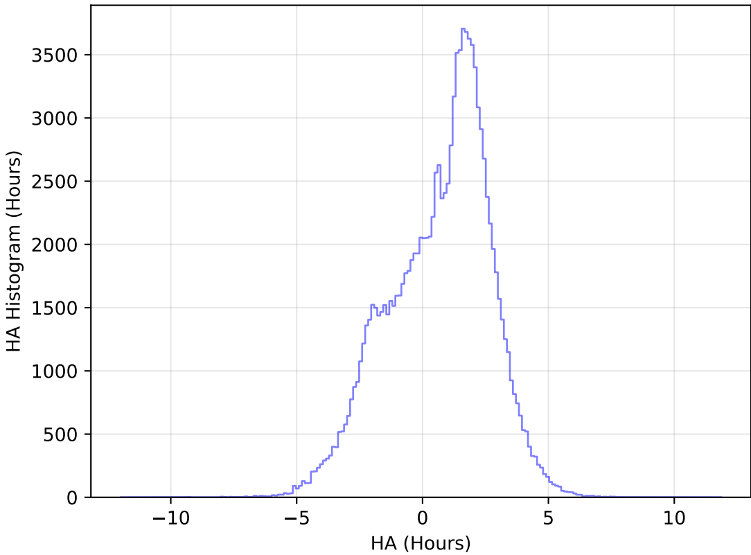
too_elab_r64_d3_ugrizy_v3.4_10yrs WFD u band: HA Histogram
