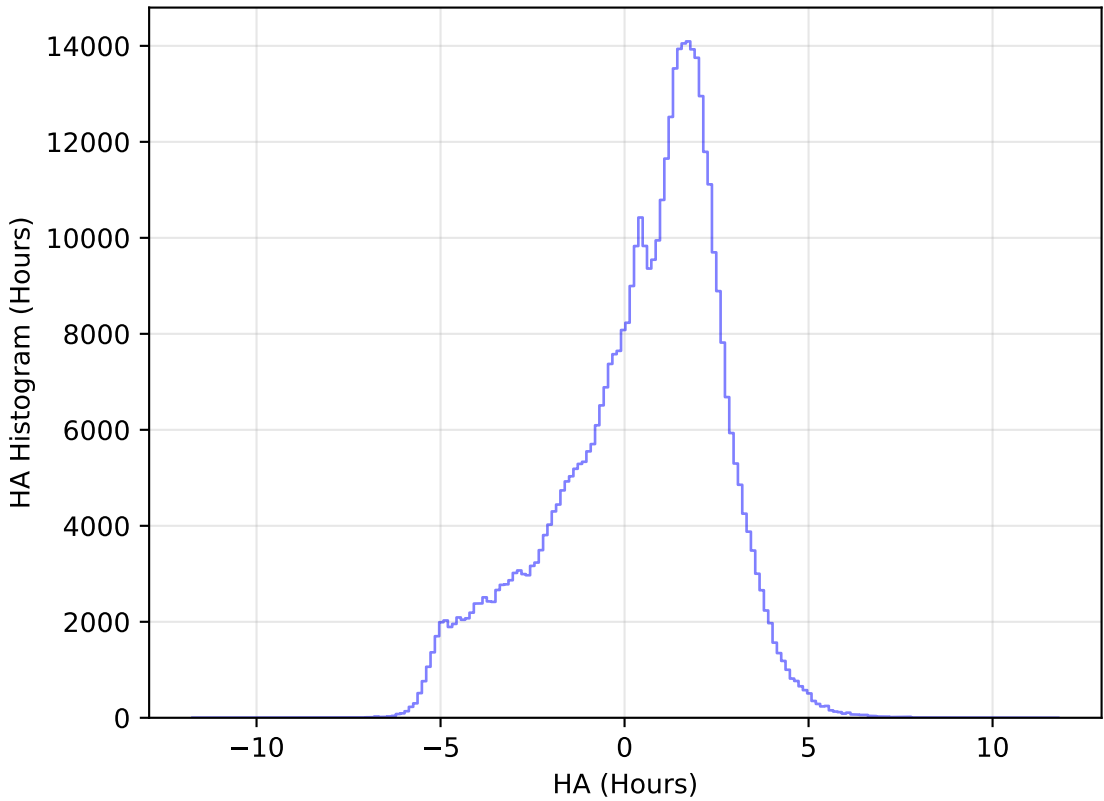
too_elab_r64_d3_ugrizy_v3.4_10yrs WFD r band: HA Histogram
