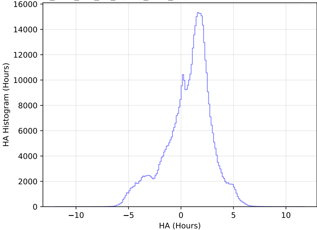
too_elab_r64_d3_ugrizy_v3.4_10yrs WFD i band: HA Histogram
