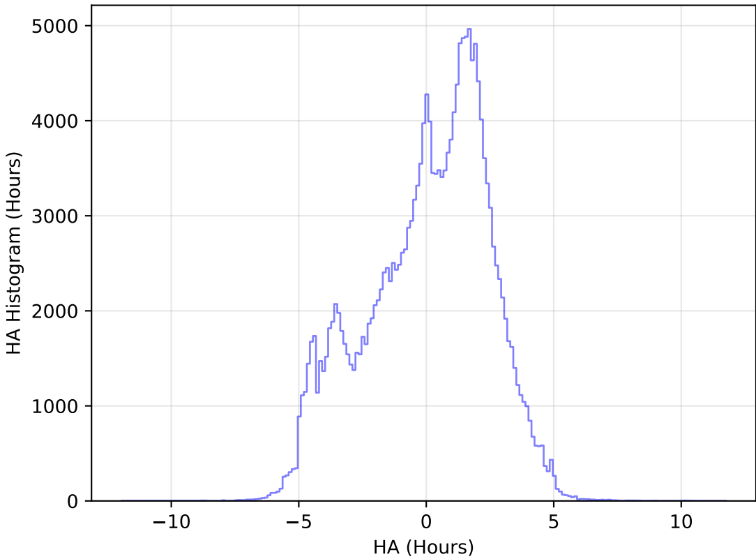
too_elab_r64_d3_ugrizy_v3.4_10yrs WFD g band: HA Histogram
