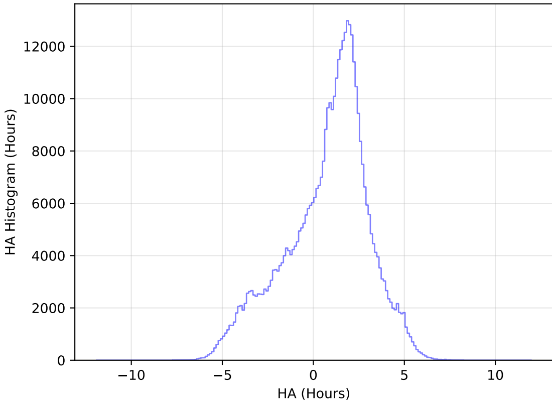
too_elab_r64_d3_ugrizy_v3.4_10yrs All sky z band: HA Histogram
