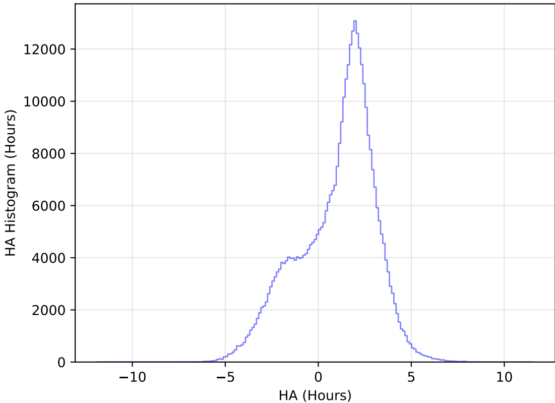
too_elab_r64_d3_ugrizy_v3.4_10yrs All sky y band: HA Histogram
