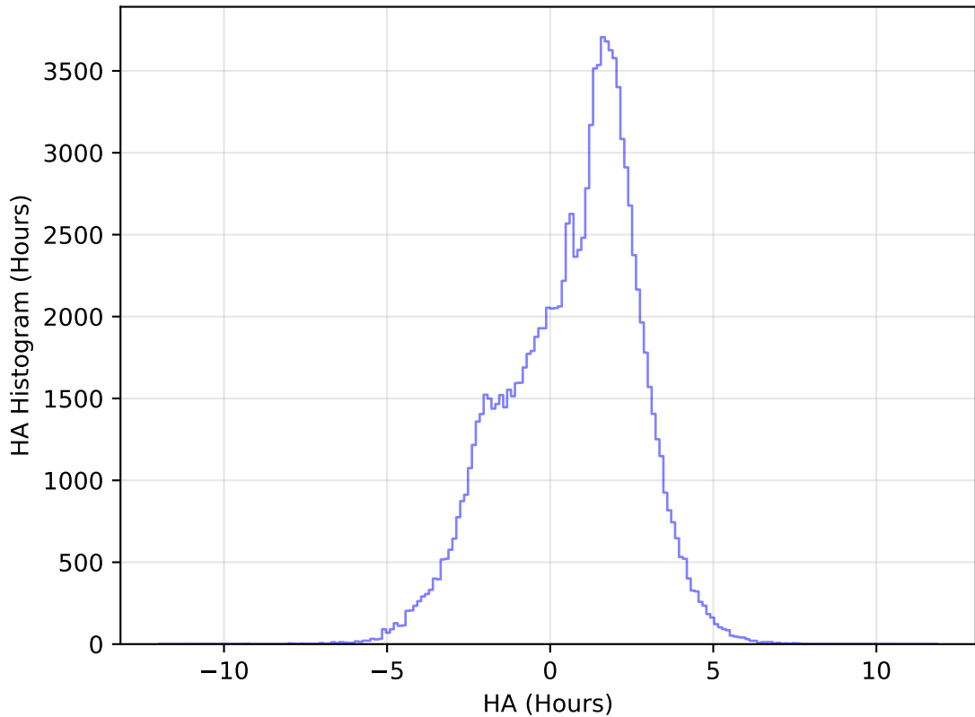
too_elab_r64_d3_ugrizy_v3.4_10yrs All sky u band: HA Histogram
