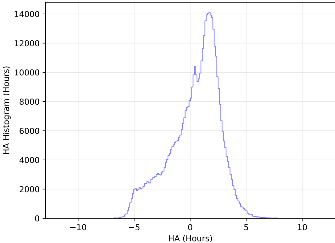
too_elab_r64_d3_ugrizy_v3.4_10yrs All sky r band: HA Histogram
