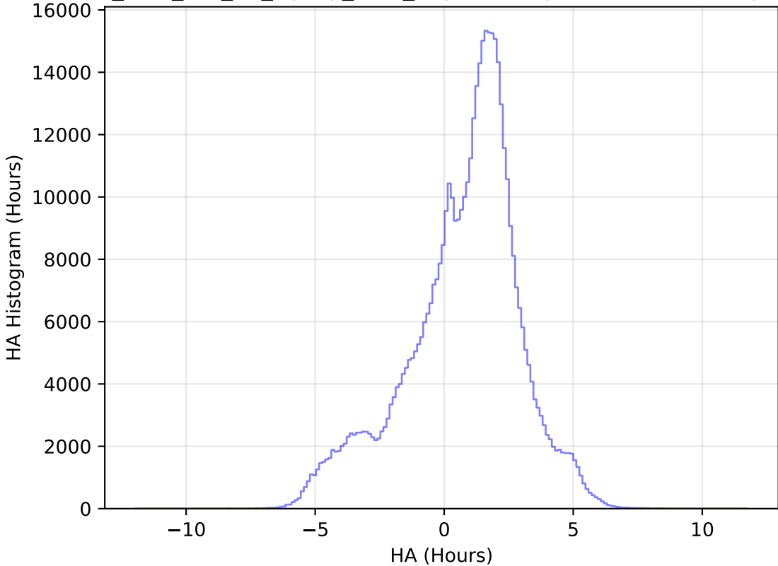
too_elab_r64_d3_ugrizy_v3.4_10yrs All sky i band: HA Histogram
