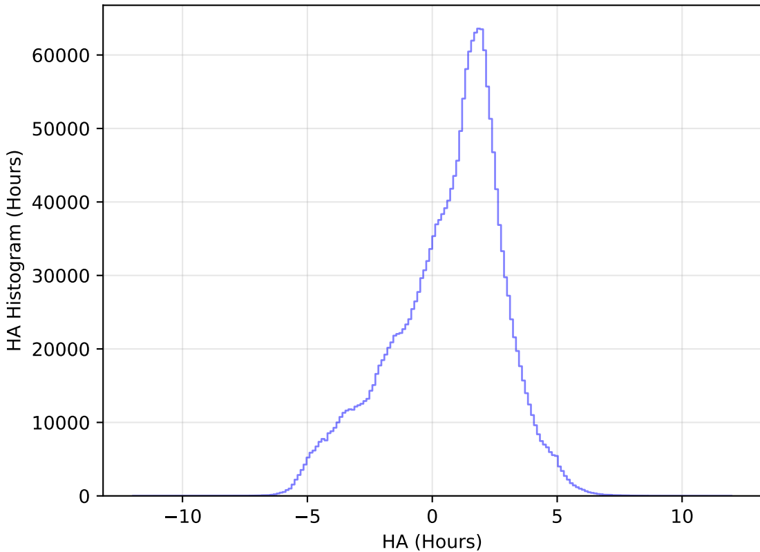
too_elab_r64_d3_ugrizy_v3.4_10yrs All sky all bands: HA Histogram
