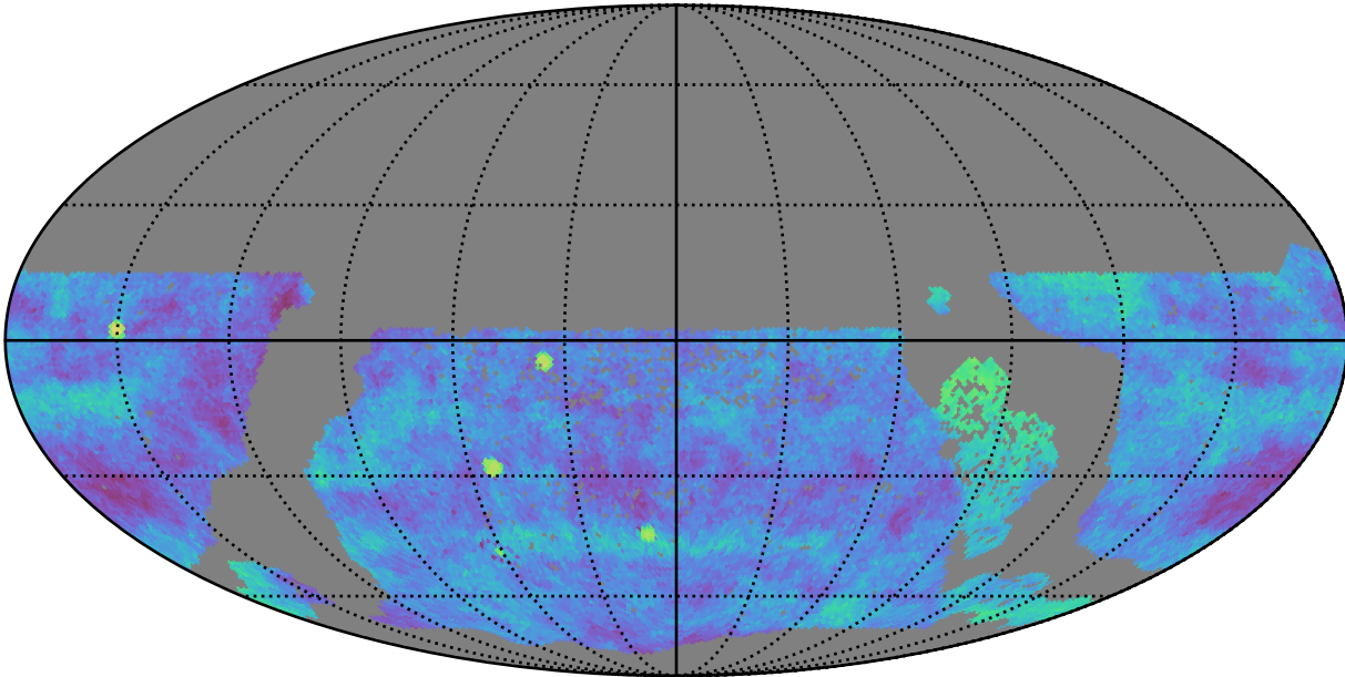
too_elab_r64_d3_ugrizy_v3.4_10yrs gri WFD: Fraction of visits in pairs (20-90 min)
