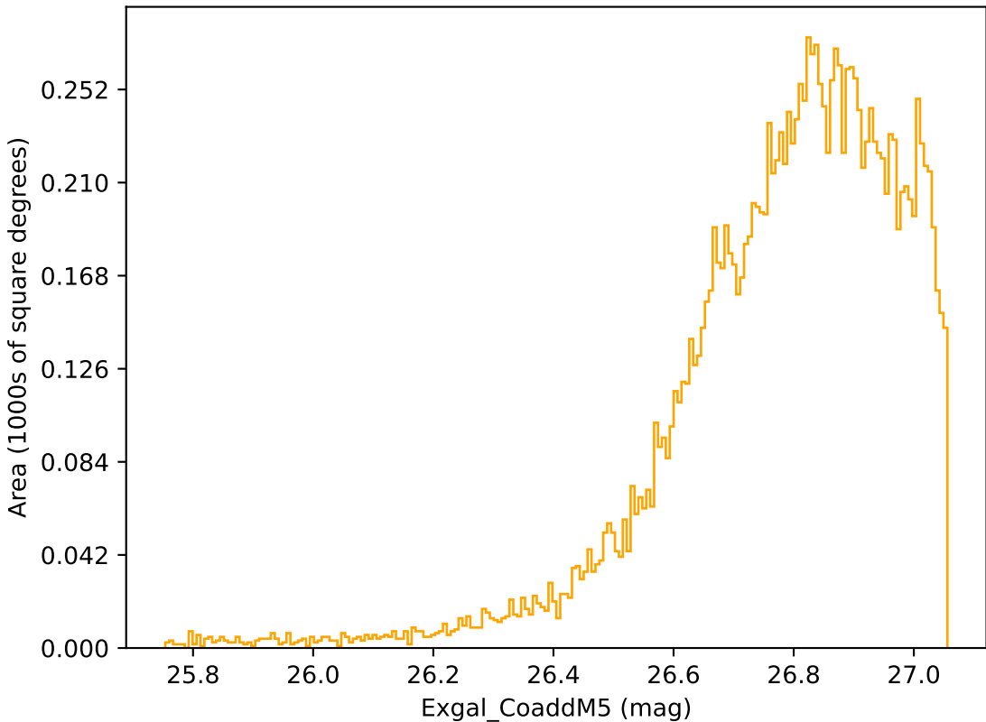
too_elab_r64_d3_ugrizy_v3.4_10yrs WFD r band: Exgal_CoaddM5
