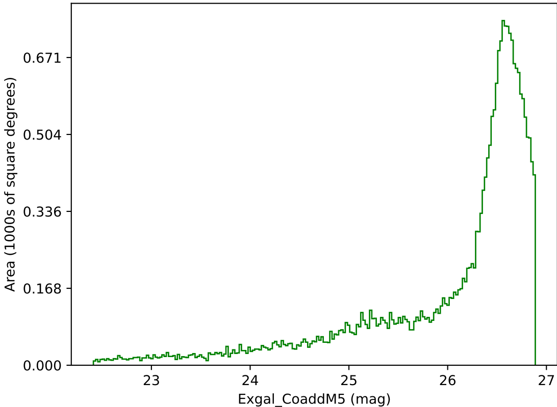
too_elab_r64_d3_ugrizy_v3.4_10yrs All sky g band: Exgal_CoaddM5
