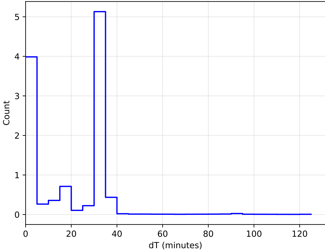
too_elab_r64_d3_ugrizy_v3.4_10yrs WFD: DeltaT Histogram 1e6
