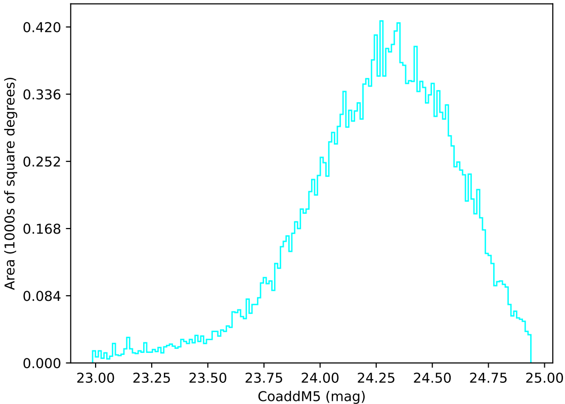
too_elab_r64_d3_ugrizy_v3.4_10yrs Yr 1 u band: CoaddM5
