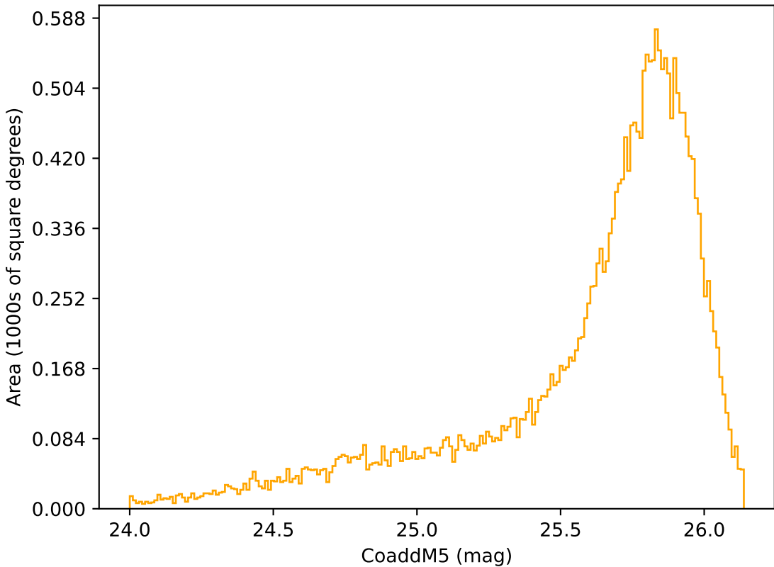
too_elab_r64_d3_ugrizy_v3.4_10yrs Yr 1 r band: CoaddM5
