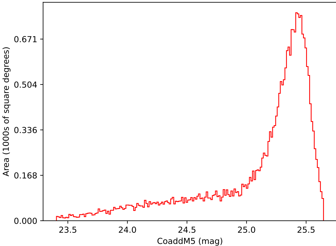
too_elab_r64_d3_ugrizy_v3.4_10yrs Yr 1 i band: CoaddM5
