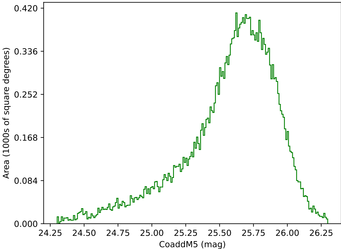
too_elab_r64_d3_ugrizy_v3.4_10yrs Yr 1 g band: CoaddM5
