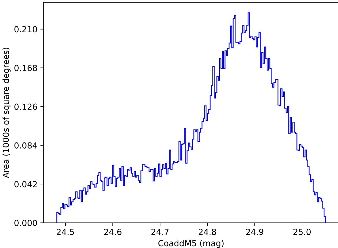
too_elab_r64_d3_ugrizy_v3.4_10yrs WFD y band: CoaddM5
