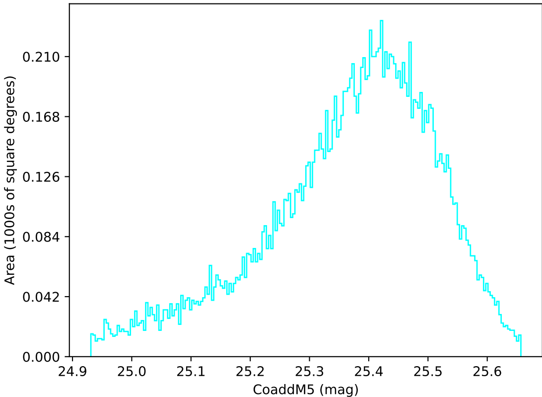
too_elab_r64_d3_ugrizy_v3.4_10yrs WFD u band: CoaddM5
