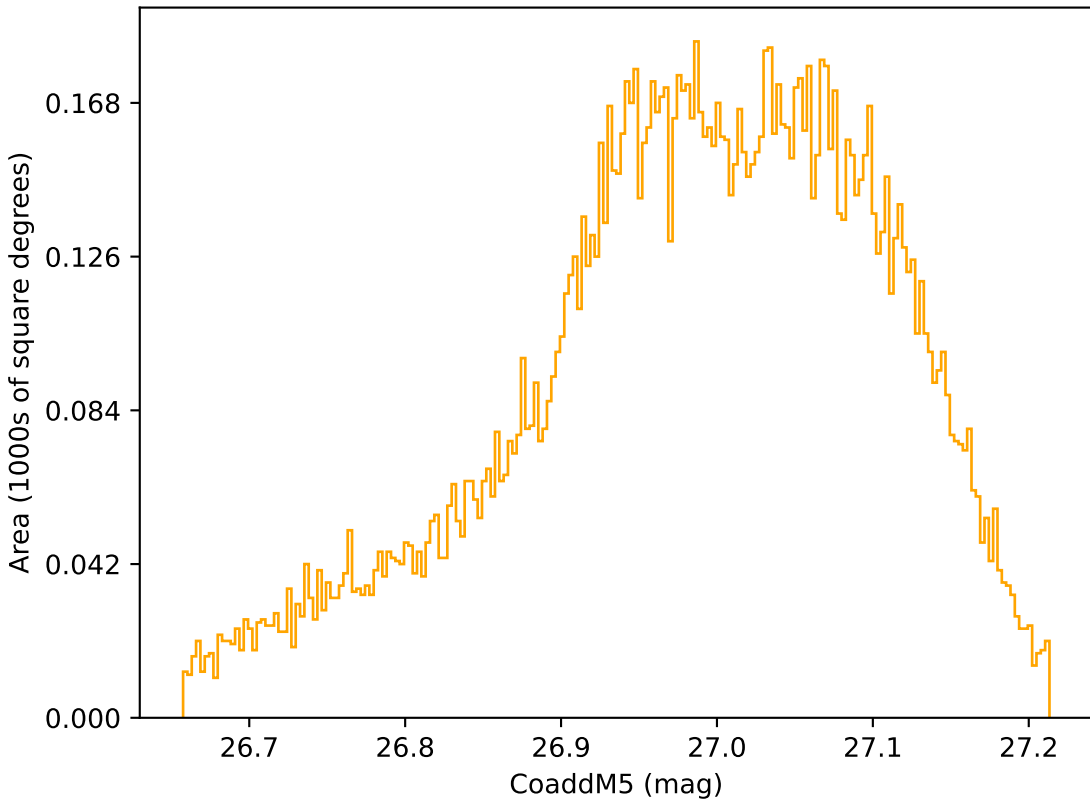
too_elab_r64_d3_ugrizy_v3.4_10yrs WFD r band: CoaddM5
