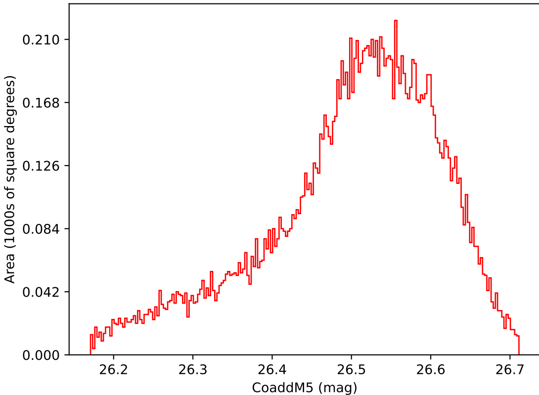
too_elab_r64_d3_ugrizy_v3.4_10yrs WFD i band: CoaddM5
