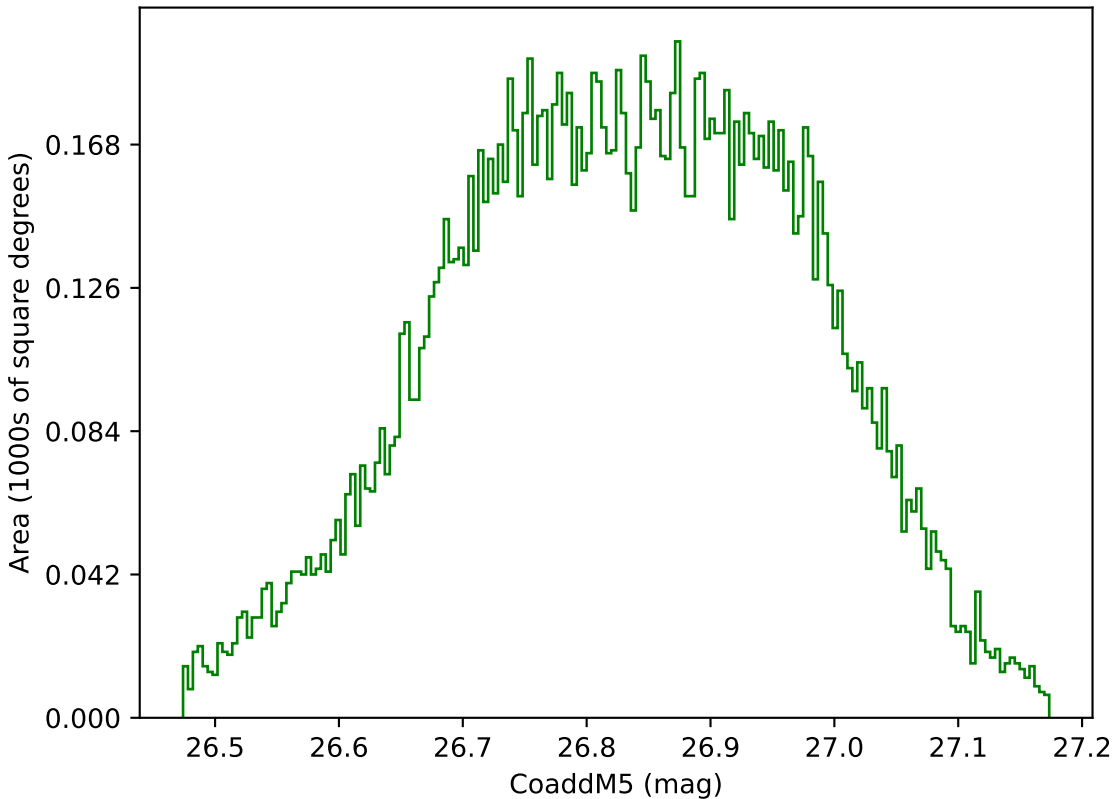
too_elab_r64_d3_ugrizy_v3.4_10yrs WFD g band: CoaddM5
