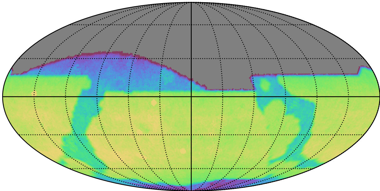
too_elab_r64_d3_ugrizy_v3.4_10yrs All sky z band: CoaddM5
