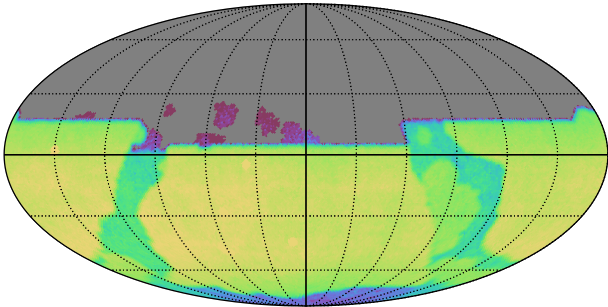
too_elab_r64_d3_ugrizy_v3.4_10yrs All sky y band: CoaddM5
