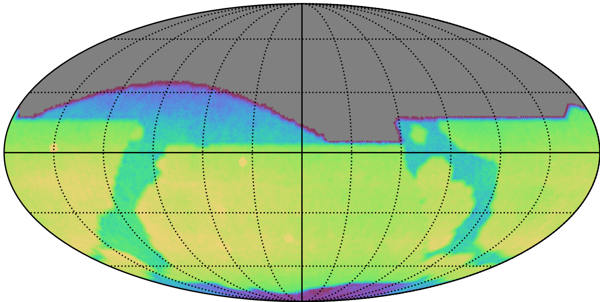
too_elab_r64_d3_ugrizy_v3.4_10yrs All sky r band: CoaddM5
