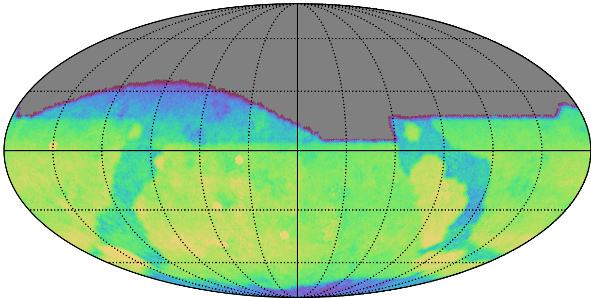
too_elab_r64_d3_ugrizy_v3.4_10yrs All sky g band: CoaddM5
