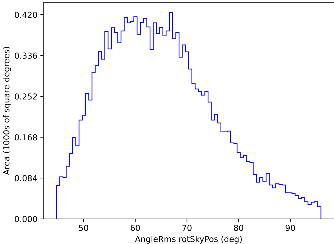
too_elab_r64_d3_ugrizy_v3.4_10yrs WFD u band: AngleRms rotSkyPos
