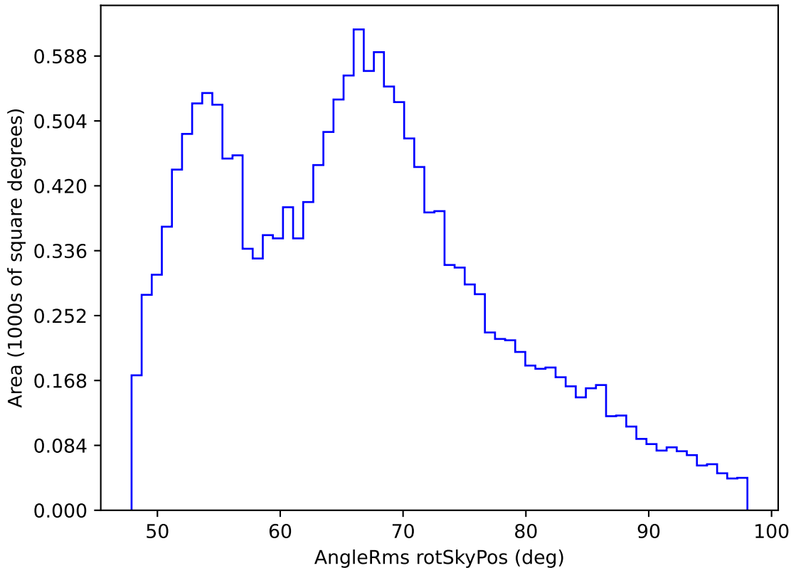
too_elab_r64_d3_ugrizy_v3.4_10yrs WFD r band: AngleRms rotSkyPos
