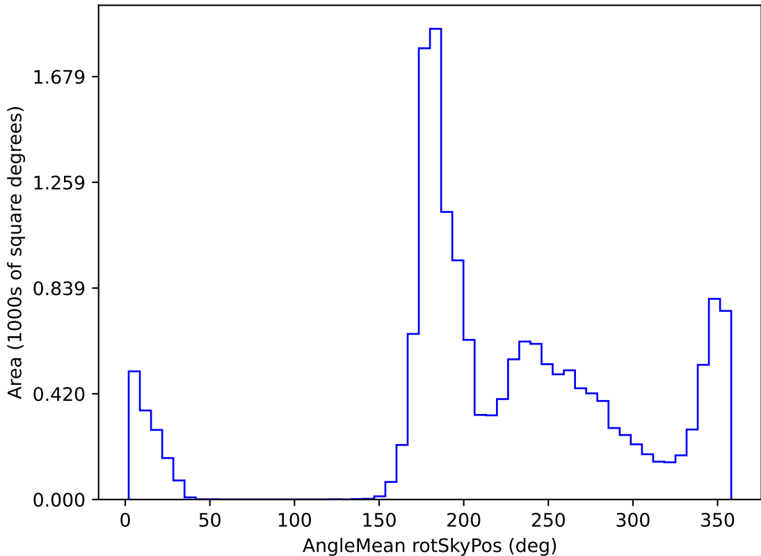
too_elab_r64_d3_ugrizy_v3.4_10yrs WFD i band: AngleMean rotSkyPos
