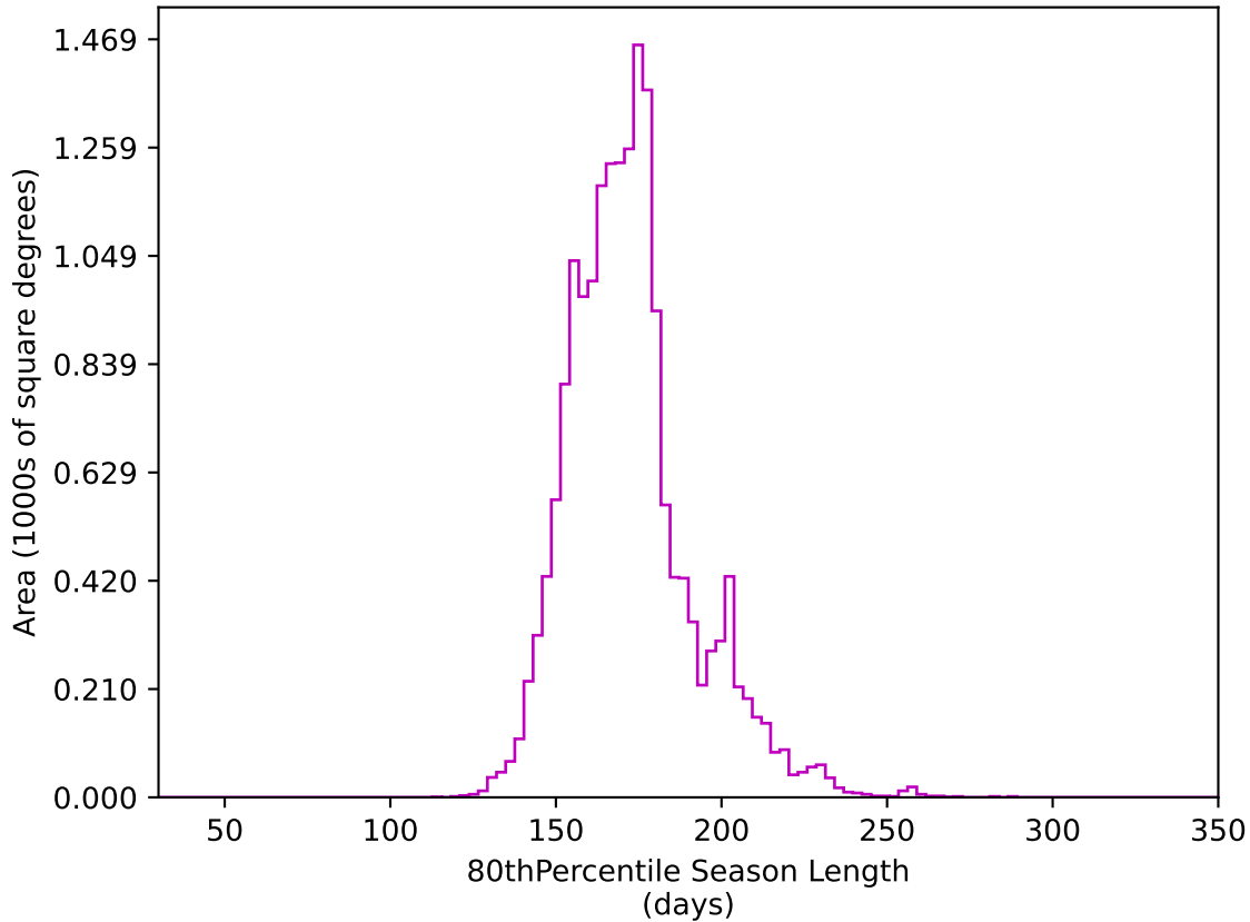
too_elab_r64_d3_ugrizy_v3.4_10yrs WFD z band: 80thPercentile Season Length
