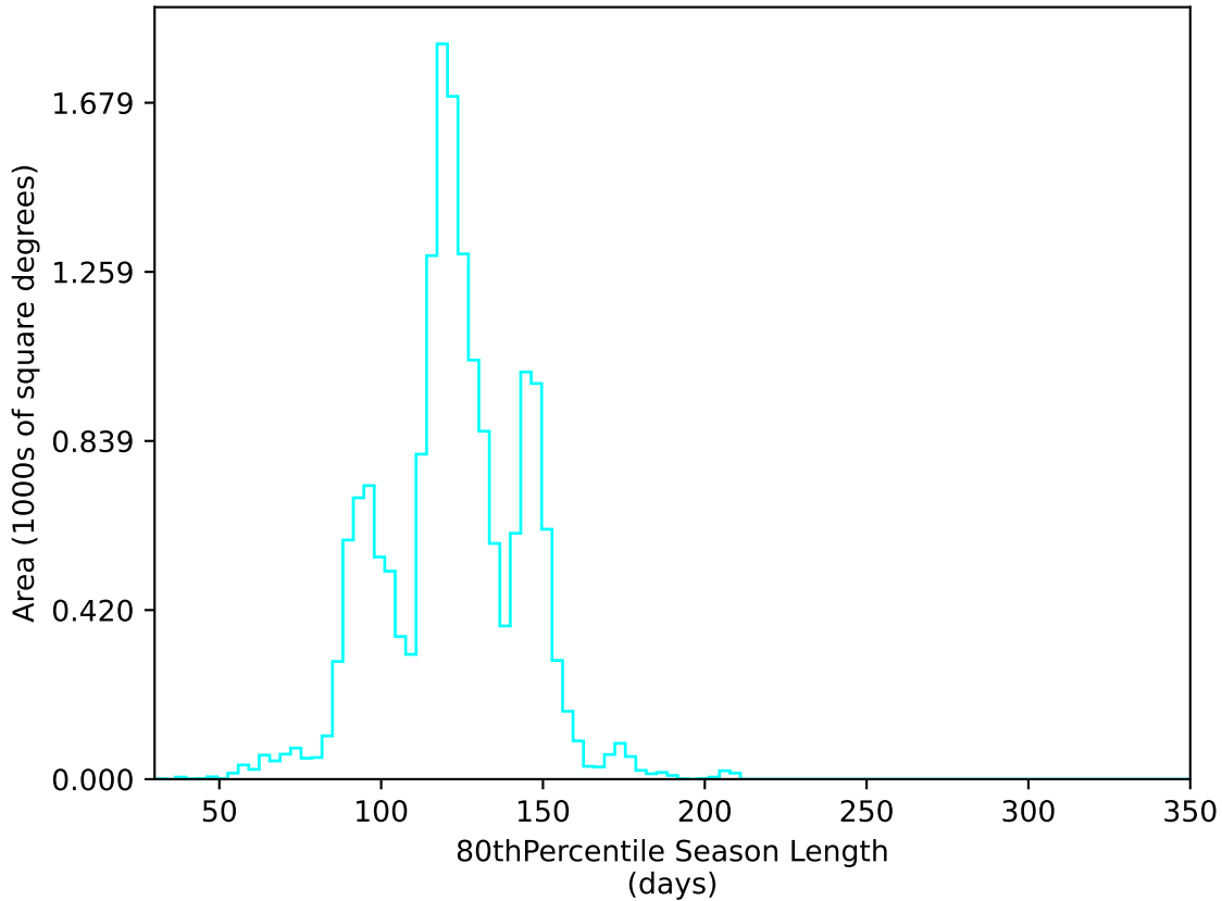
too_elab_r64_d3_ugrizy_v3.4_10yrs WFD u band: 80thPercentile Season Length
