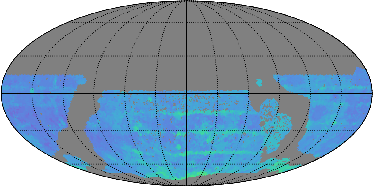
too_elab_r64_d3_ugrizy_v3.4_10yrs WFD r band: 80thPercentile Season Length
