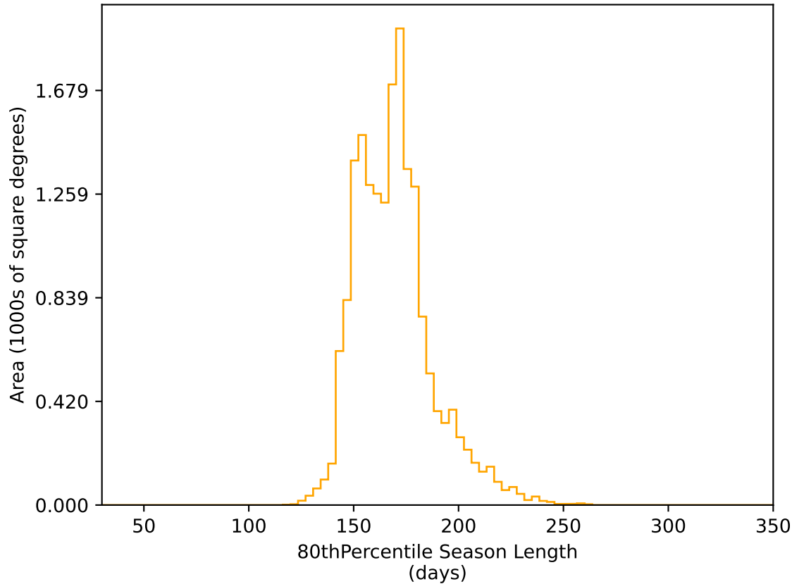
too_elab_r64_d3_ugrizy_v3.4_10yrs WFD r band: 80thPercentile Season Length
