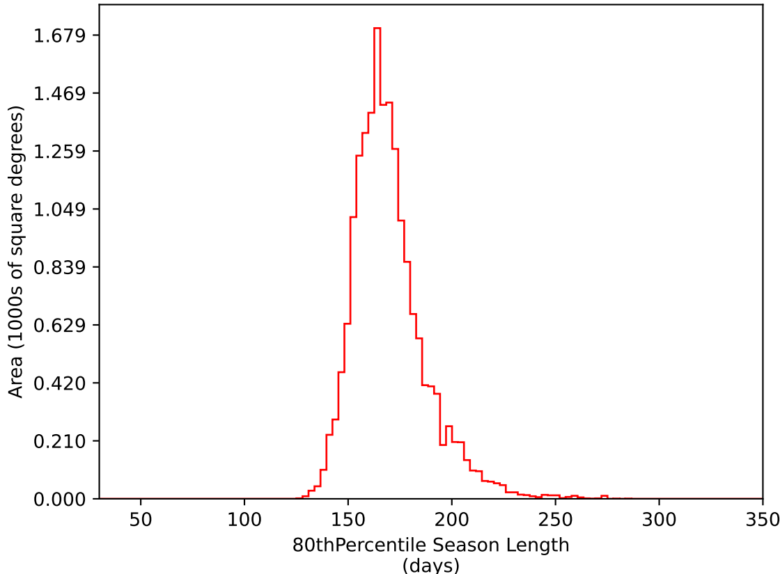
too_elab_r64_d3_ugrizy_v3.4_10yrs WFD i band: 80thPercentile Season Length
