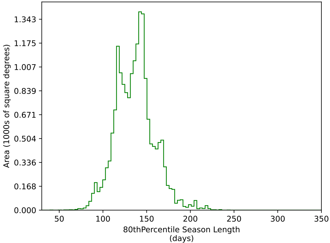
too_elab_r64_d3_ugrizy_v3.4_10yrs WFD g band: 80thPercentile Season Length
