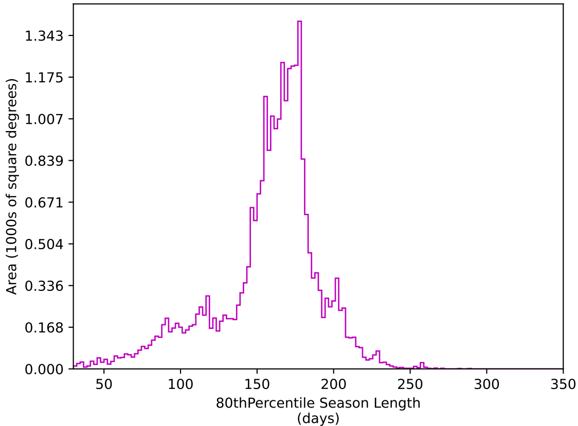
too_elab_r64_d3_ugrizy_v3.4_10yrs All sky z band: 80thPercentile Season Length
