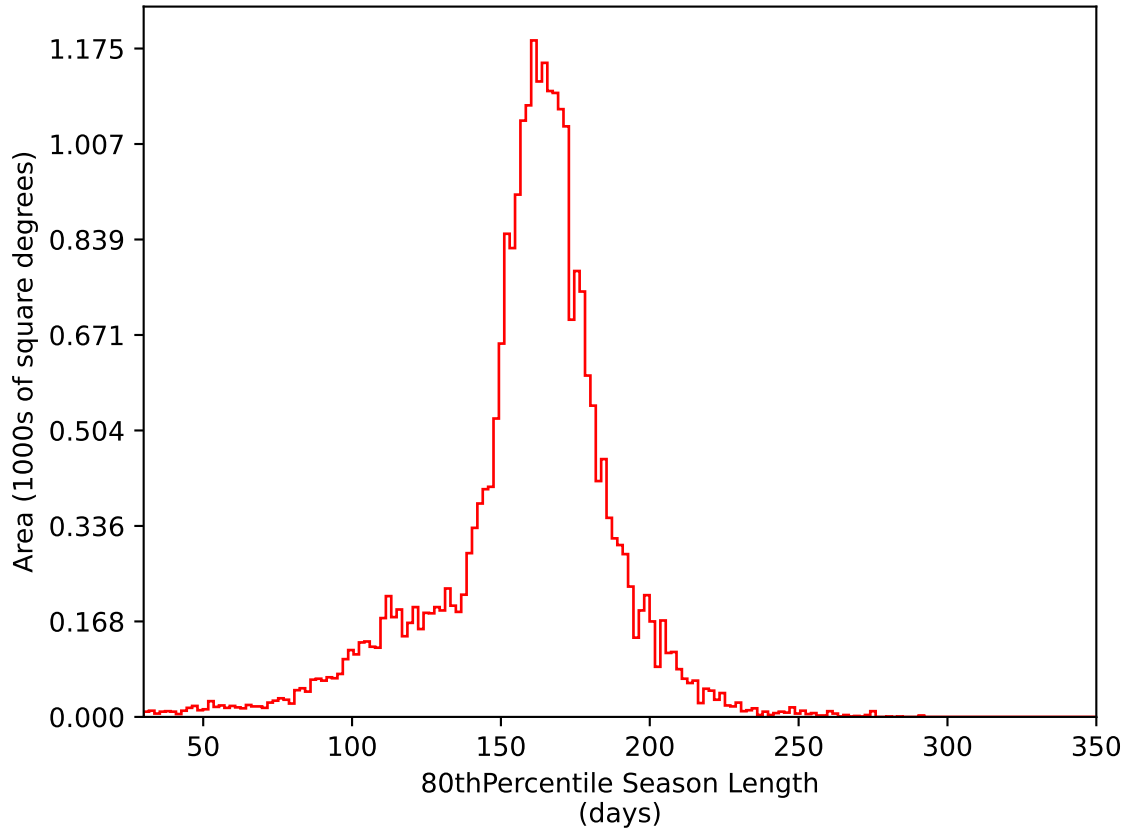
too_elab_r64_d3_ugrizy_v3.4_10yrs All sky i band: 80thPercentile Season Length
