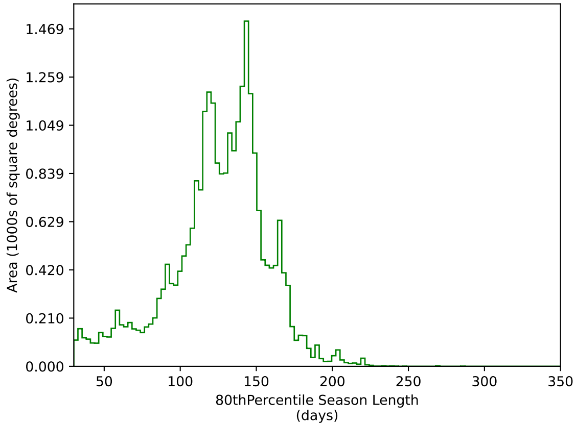
too_elab_r64_d3_ugrizy_v3.4_10yrs All sky g band: 80thPercentile Season Length
