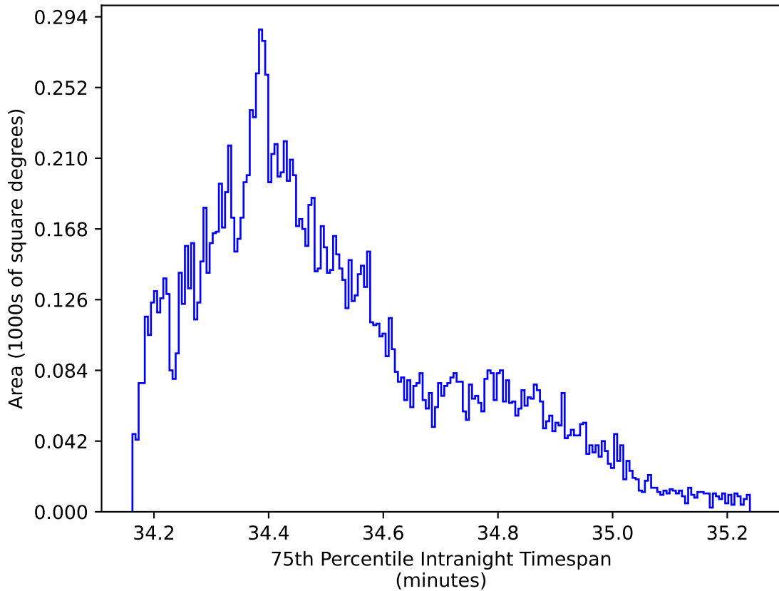
too_elab_r64_d3_ugrizy_v3.4_10yrs WFD zy bands: 75th Percentile Intranight Timespan
