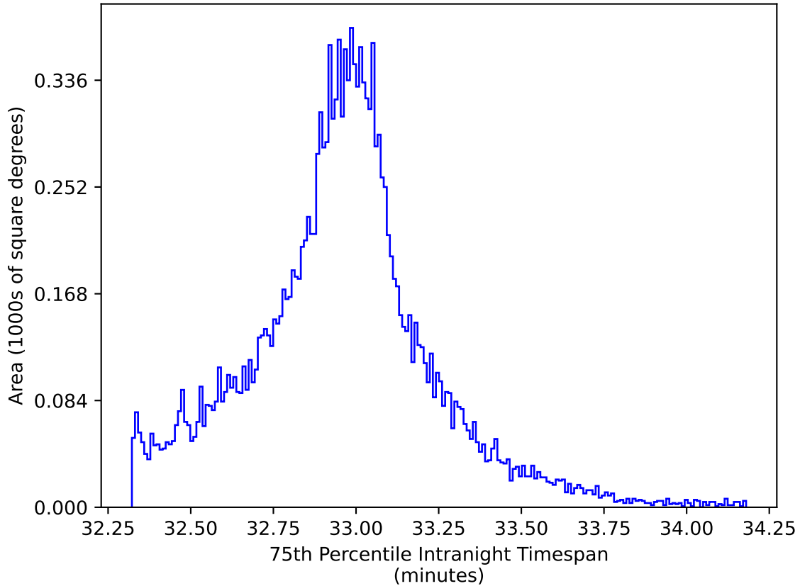
too_elab_r64_d3_ugrizy_v3.4_10yrs WFD y band: 75th Percentile Intranight Timespan
