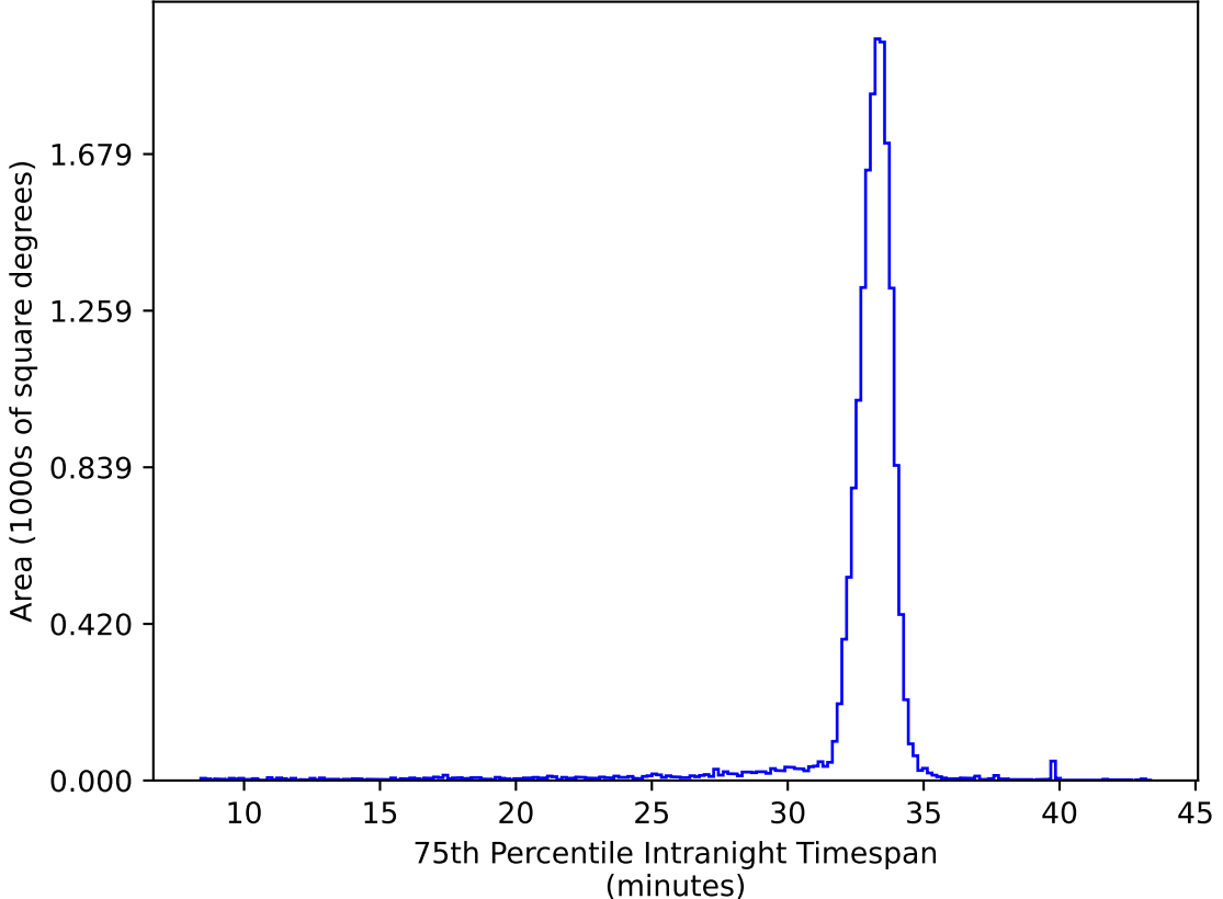
too_elab_r64_d3_ugrizy_v3.4_10yrs WFD ug bands: 75th Percentile Intranight Timespan
