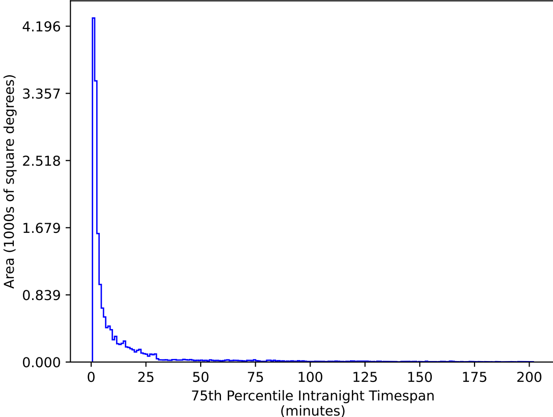
too_elab_r64_d3_ugrizy_v3.4_10yrs WFD u band: 75th Percentile Intranight Timespan
