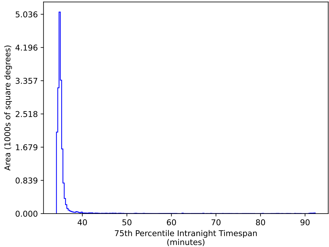
too_elab_r64_d3_ugrizy_v3.4_10yrs WFD ri bands: 75th Percentile Intranight Timespan
