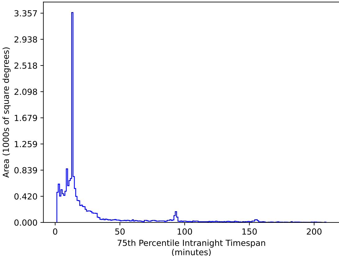
too_elab_r64_d3_ugrizy_v3.4_10yrs WFD i band: 75th Percentile Intranight Timespan
