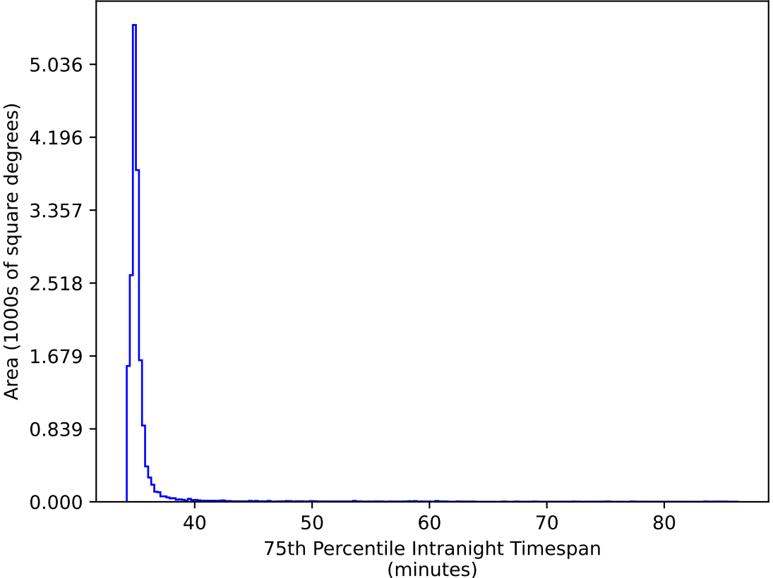
too_elab_r64_d3_ugrizy_v3.4_10yrs WFD gr bands: 75th Percentile Intranight Timespan
