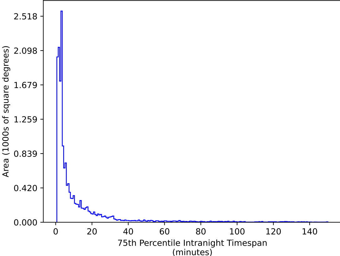
too_elab_r64_d3_ugrizy_v3.4_10yrs WFD g band: 75th Percentile Intranight Timespan
