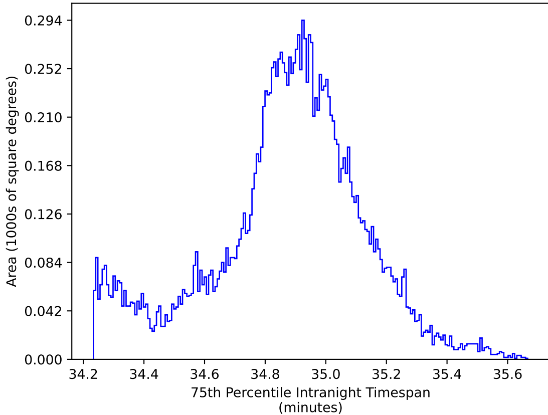
too_elab_r64_d3_ugrizy_v3.4_10yrs WFD all bands: 75th Percentile Intranight Timespan
