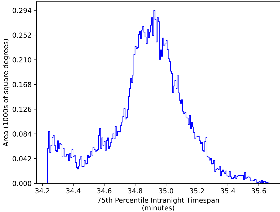
too_elab_r64_d3_ugrizy_v3.4_10yrs WFD: 75th Percentile Intranight Timespan
