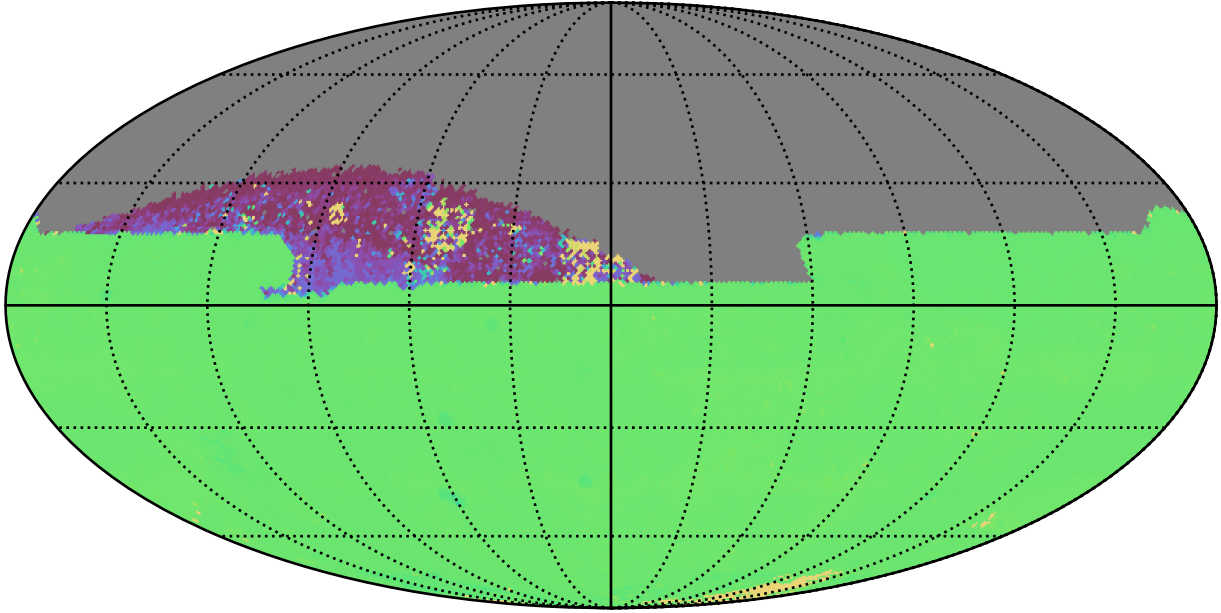
too_elab_r64_d3_ugrizy_v3.4_10yrs All sky zy bands: 75th Percentile Intranight Timespan
